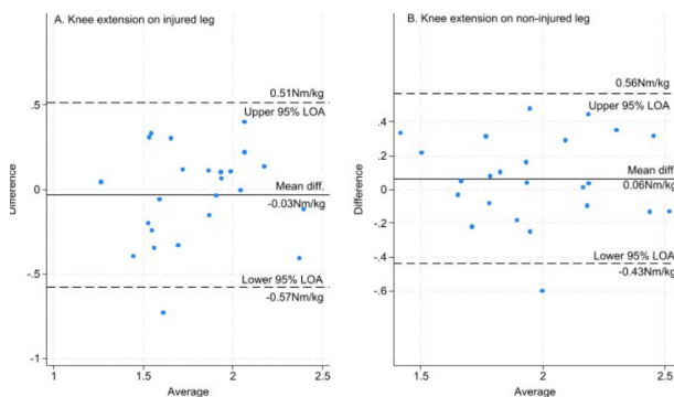
Figure 4 A and B. Bland-Altman plots for the ForceFrame MVIC knee extension of the injured leg (A) and non-injured leg (B)
