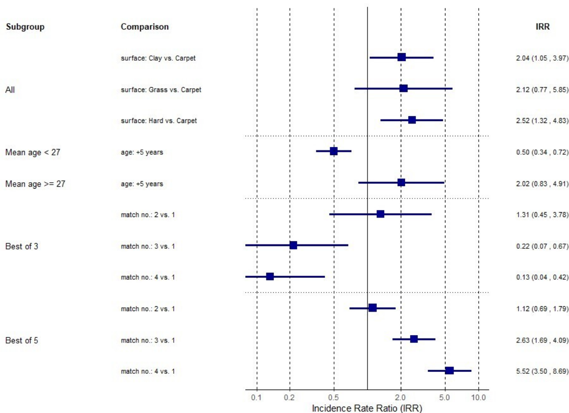
Figure 2. Incidence rate ratio for different factors of Davis Cup matches.
